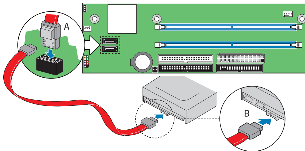
Figure 19. Connecting the Serial ATA Cable
